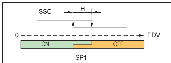
Fig. 2: Normally closed = high active
