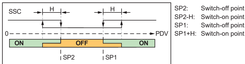
Fig. 3: Normally open = low active
