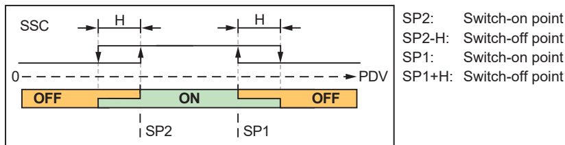
Fig. 4: Normally closed = high active
