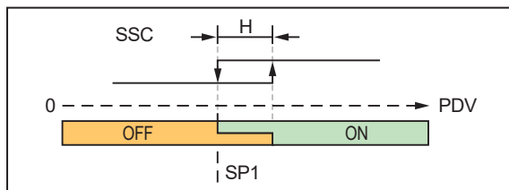
Fig. 1: Normally open = low active (factory setting)
